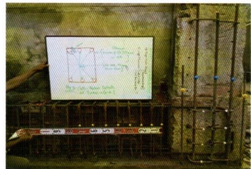
Insertion of New Column and Beam
