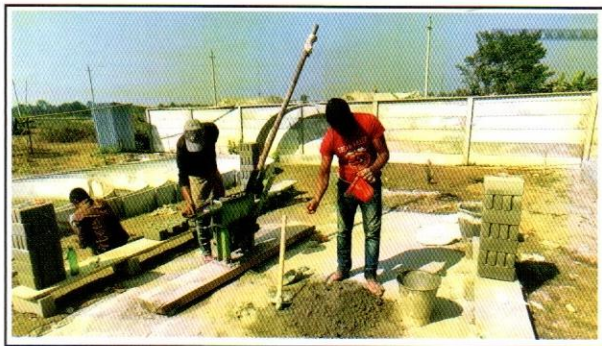
Fig 1: Production of CSEB at Site
