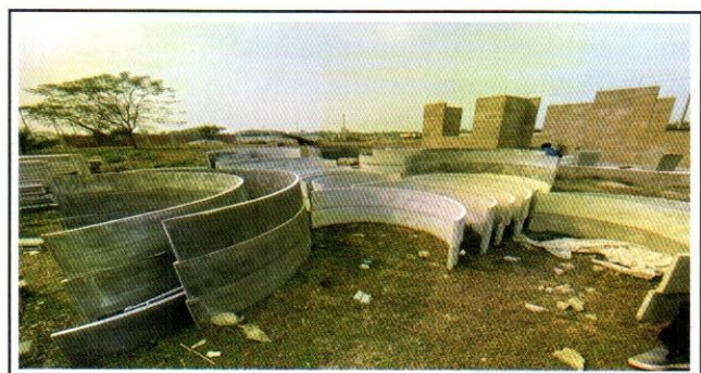
Fig 4: Ferrocement pre-cast vault roof strips
