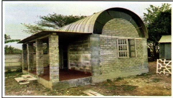
Fig 5: External View of Model House
