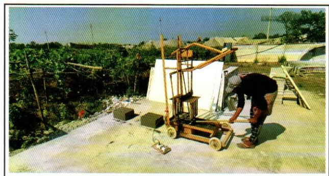
Fig 2: Production of Concrete Block at Site
