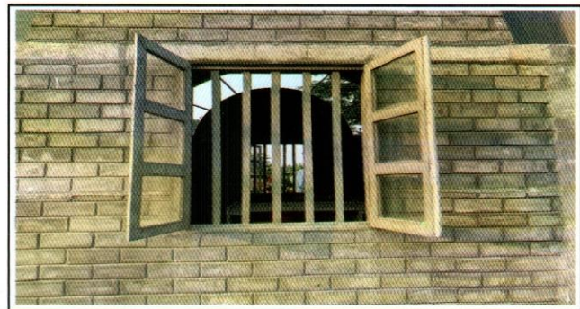
Fig. 8: Ferrocement Window Frame & Shutter
